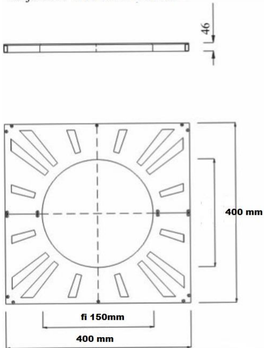
varijanta 1: 400x400x2 / fi 150mm
