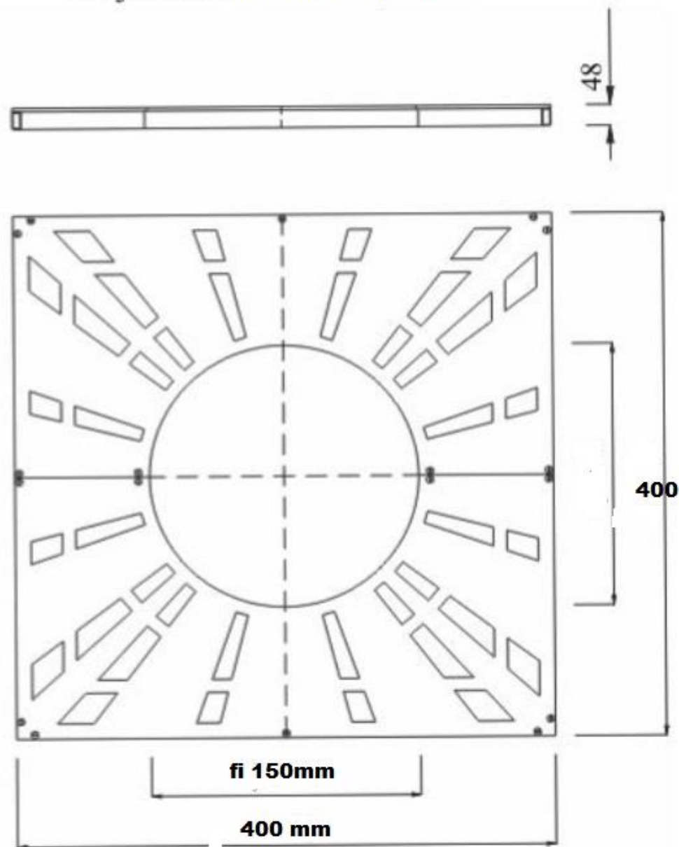
varijanta 2: 400x400x2 / fi150mm
